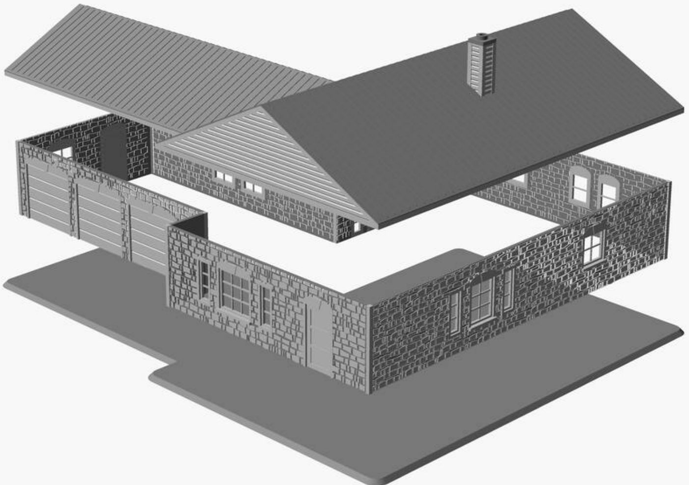
EXPLODED ASSEMBLY VIEW
